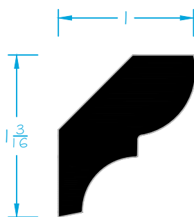
Bed Mould - 8ft D75 - 9/16" x 1 - 9/16"
