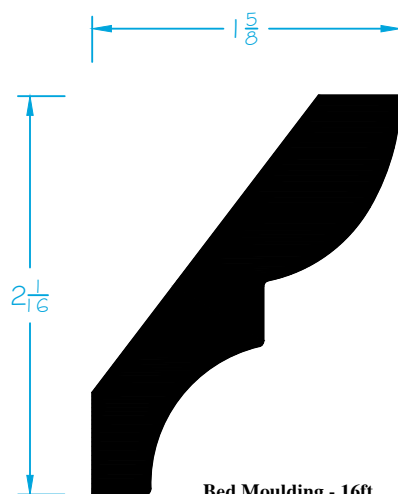
Bed Moulding - 16ft D70 - 9/16" x 2-5/8"
