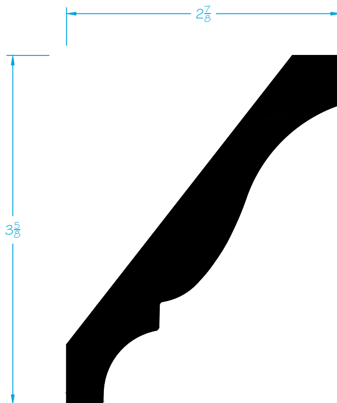
Crown Moulding - 16ft D47 - 11/16" x 4-5/8"
