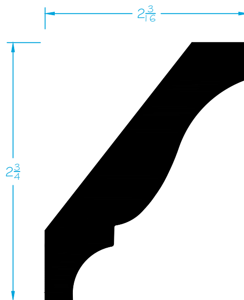
Crown Moulding - 16ft D49 - 11/16" x 3-1/2"
