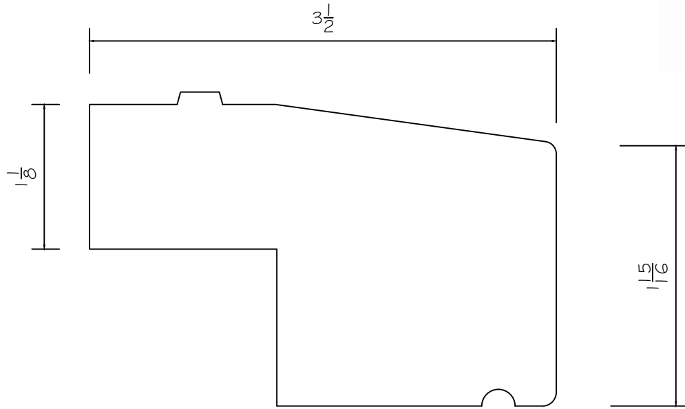
DSC-044 -B 2 - 3/8" x 3 -1/2"
