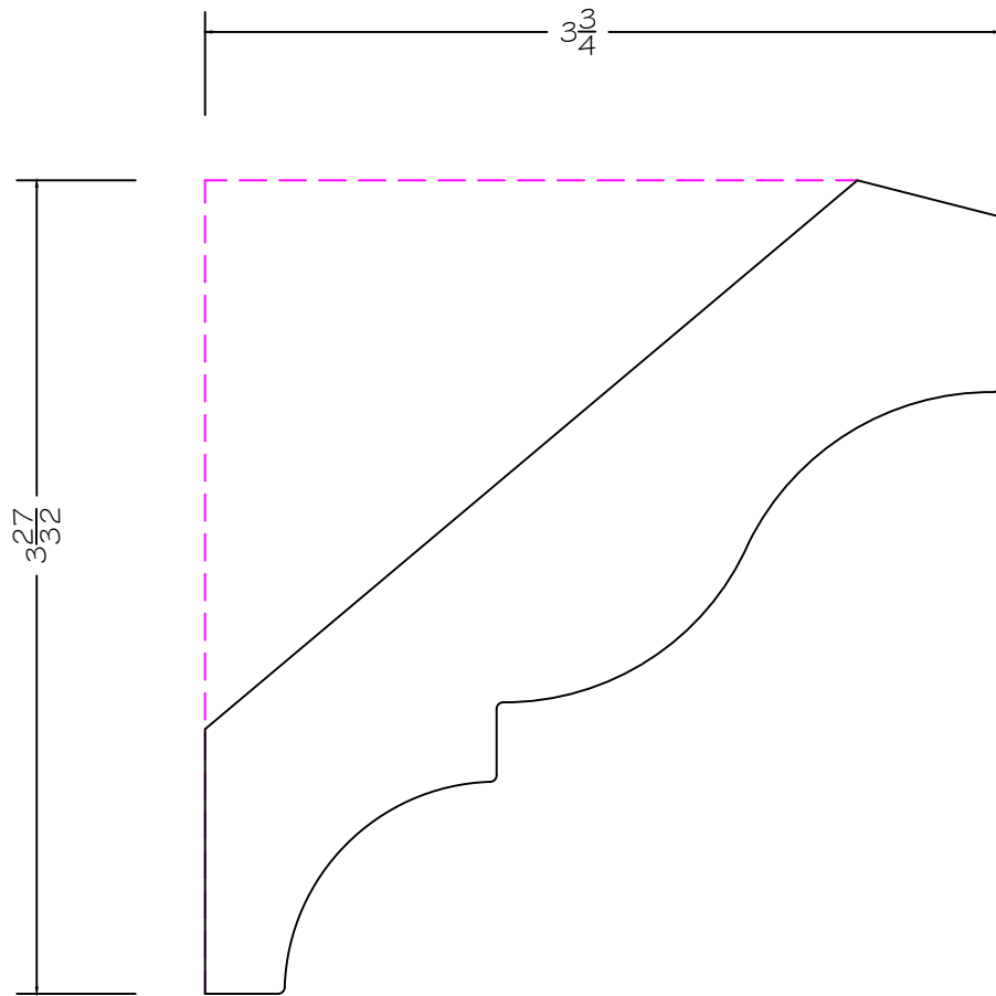
DSC-217 1-1/8" x 5-1/4"
