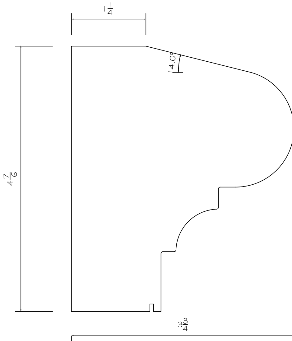
DSC-127 4 - 7/16" x 3 - 23/32"
