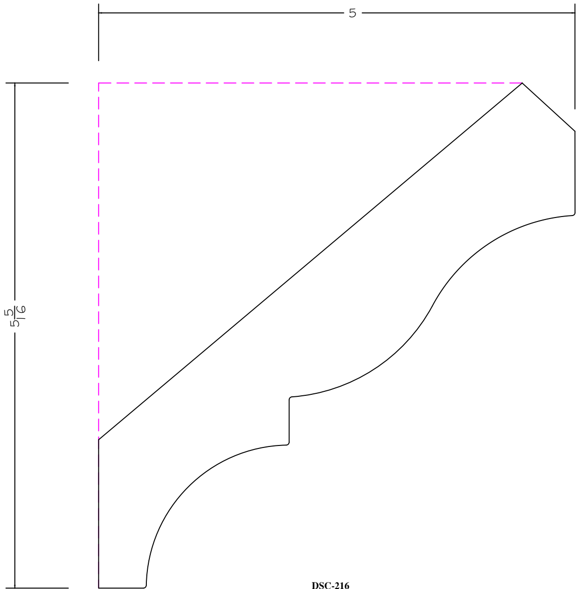
DSC-216 1 - \frac{7}{16} " x 6 - \frac{7}{8} "
