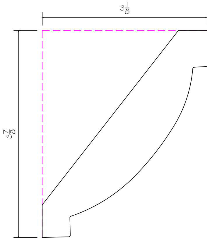
DSC-183 1-1/16" x 5"
