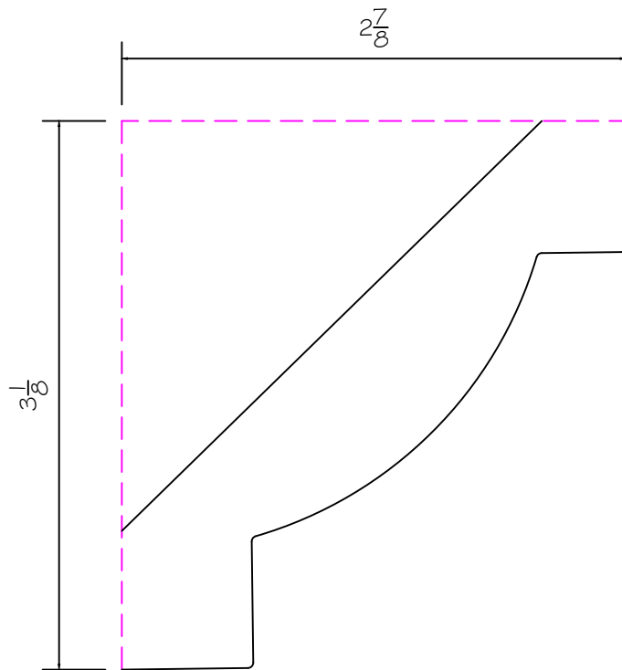
DSC-117 1" x 4-1/4"
