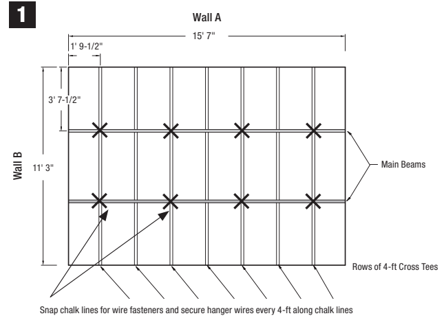
Grid layout, example: main beams, 4-ft tees and hanger wire.
