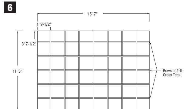
Example of complete installed grid system.
